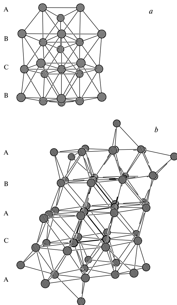
Fig. 9. Metal cores with a mixed f.c.c./h.c.p. packing: (a) [\text{Rh}_{22}(\text{CO})_{37}]^{4-} (ABCB) and (b) \text{Pd}_{54}(\text{CO})_{40}(\text{PEt}_3)_{14} (ABACA). 73 The motifs of stacking of the layers are denoted; in \text{Pd}_{54}(\text{CO})_{40}(\text{PEt}_3)_{14} , the six-atom inner fragment is marked.
