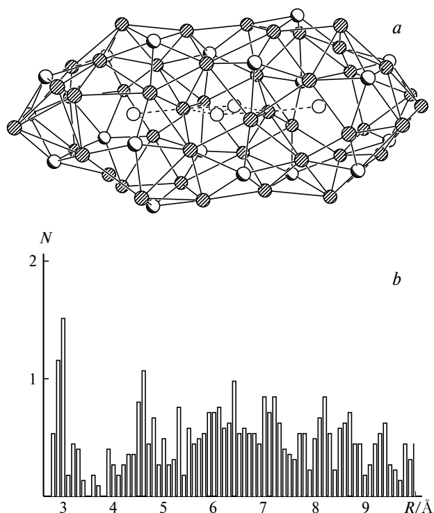
Fig. 17. Structure (a) and the histogram of the Ag—Ag distances (b) of the shell cluster \text{Ag}_{44}(\text{PPh})_{18}(\text{PhPSiMe}_3)_2\text{Cl}_5(\text{PPr}^n)_3)_{12}@\text{AgCl}_2 . 95 The disordered positions of the Cl atoms inside the polyhedron are represented by empty circles.
