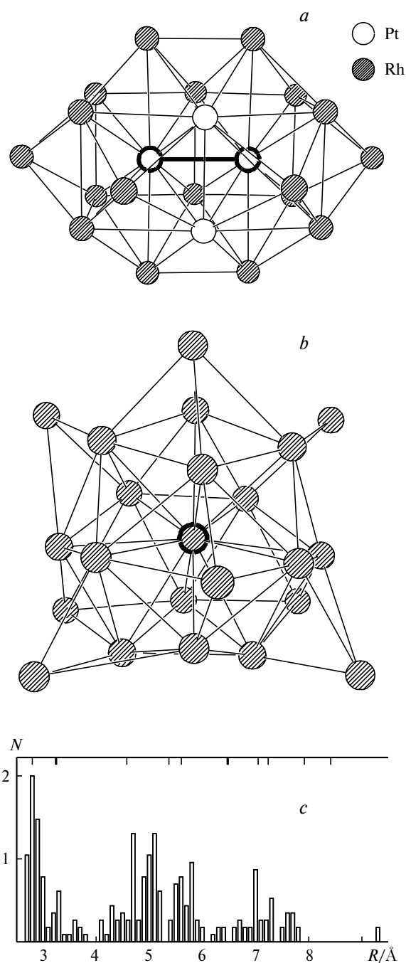
Fig. 10. Metal cores with a b.c.c. packing: (a) [\text{Pt}_4\text{Rh}_{18}(\text{CO})_{35}]^{4-52} and (b) \text{Pd}_{23}(\text{CO})_{20}(\text{PEt}_3)_8 56 (interstitial atoms are marked); (c) histogram of the Pd—Pd interatomic distances in \text{Pd}_{23}(\text{CO})_{20}(\text{PEt}_3)_8 . The coordination sphere specific for b.c.c. are indicated by bold dashes at the top of the plot (c); the coordination spheres, which are present also in f.c.c. and/or h.c.p. packings, are shown by thin dashes.
