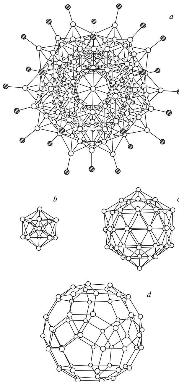
Fig. 14. Multi-shell structure of the metal core of \text{Pd}_{145}(\text{CO})_{60}(\text{PEt}_3)_{30} . 97 ( a ) overall view of the cluster without CO ligands, the P atoms of the phosphine ligands are dashed, ( b ) inner centered icosahedron \text{Pd}_{13} , ( c ) second icosahedral 42-atom shell, and ( d ) third 60-atom shell.
