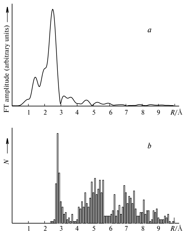
Fig. 18. Metal—metal coordination spheres in the "amorphous" \text{Pd}_{38}(\text{CO})_{28}(\text{PEt}_3)_{12} cluster 84 (a) based on the EXAFS Fourier transform (Pd K-edge) and (b) according to the histogram of the Pd—Pd interatomic distances determined by X-ray diffraction analysis. 126
