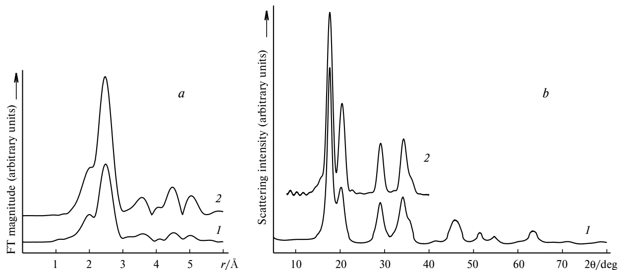
Fig. 20. ( a ) Coordination spheres in the Fourier transforms of Pd K-edge EXAFS for palladium black (1) and Pd foil (2); ( b ) X-ray diffraction pattern of Pd black (Photon Factory, BL-1B, \lambda = 0.6888 Å): 132 1, the experimental pattern; 2, the pattern calculated for the six-shell f.c.c. \text{Pd}_{923} cluster.
